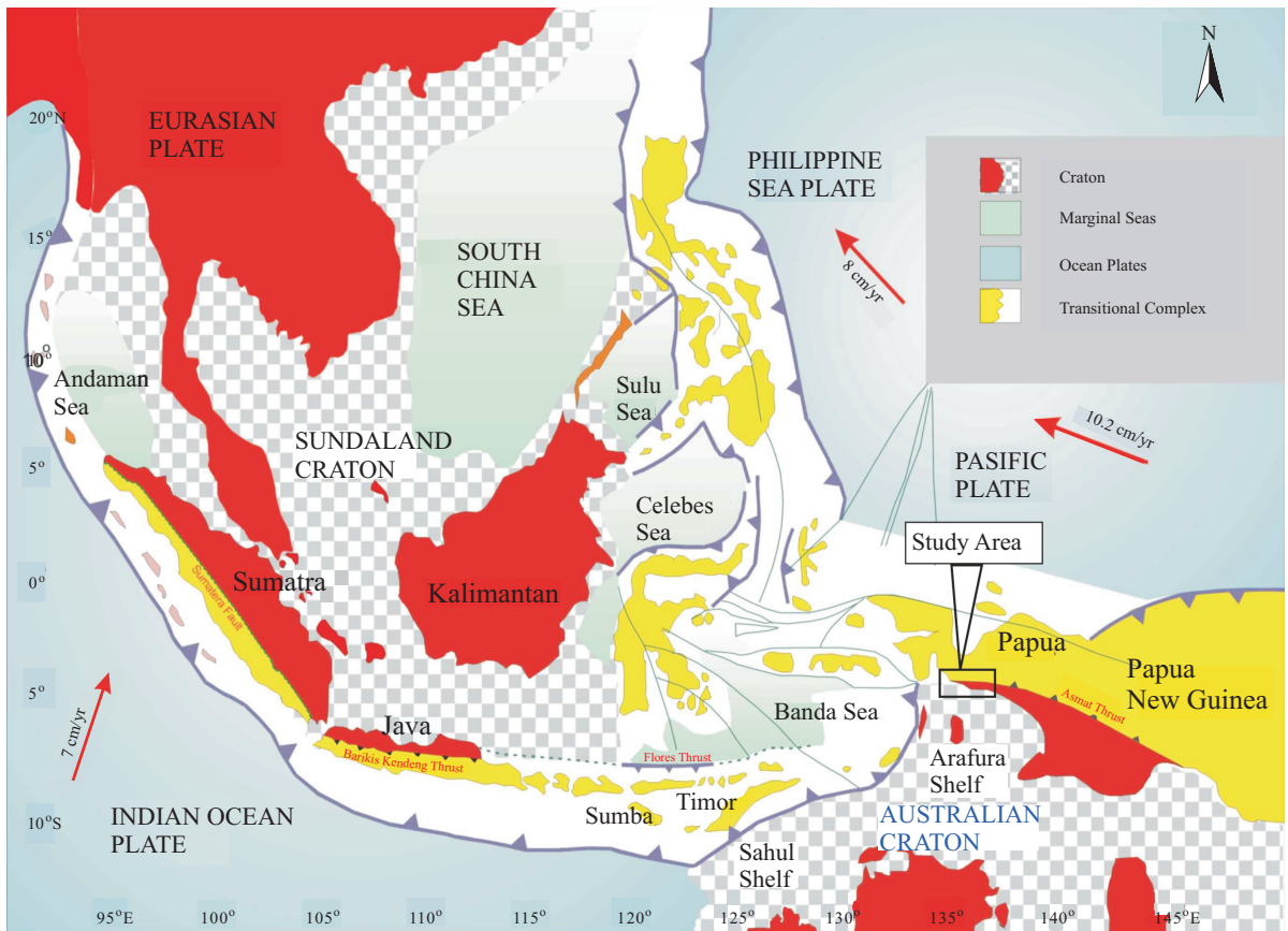
Figure 1. Tectonic framework of Indonesia (Simandjuntak and Barber, 1996). Papua (formerly Irian Jaya) lies on the Australian continental margin
