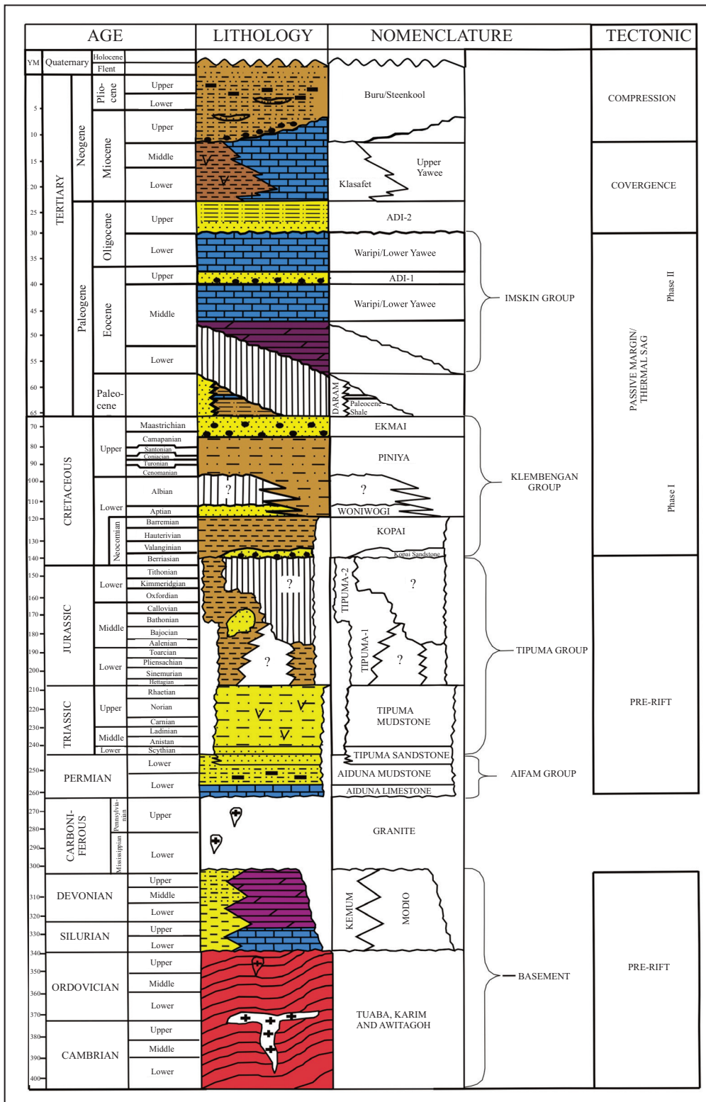
Figure 4. Tectonostratigraphy phase diagram of southern Papua and Arafura Sea area (data is derived from many sources i.e. Pieters et al. , 1983; Dow et al. , 1986 etc).
