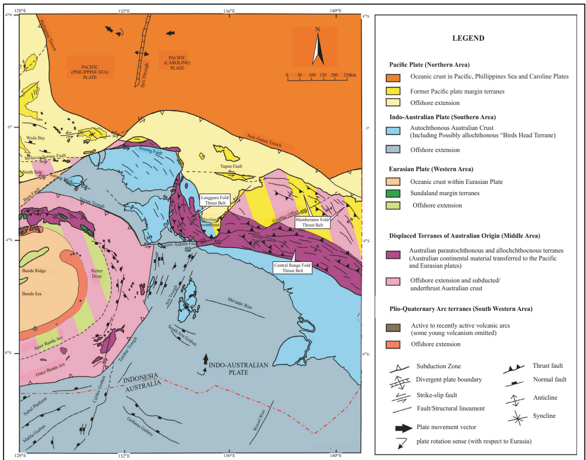
Figure 3. Regional tectonic map of eastern Indonesia (data source from KNOC, 1999; Dow et al. , 1986; Hamilton, 1979; Simandjuntak and Barber, 1996).
