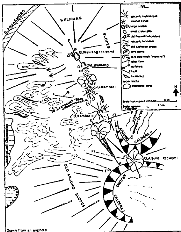
Figure 2. - The volcanic arjuno-welirang faultzone
